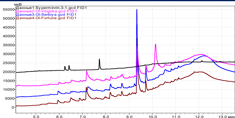
Figure 1: Chromatograms of the cypermethrin standard sample and plum extracts of the Hungarian, Serbian, and Fortuna cultivars.
