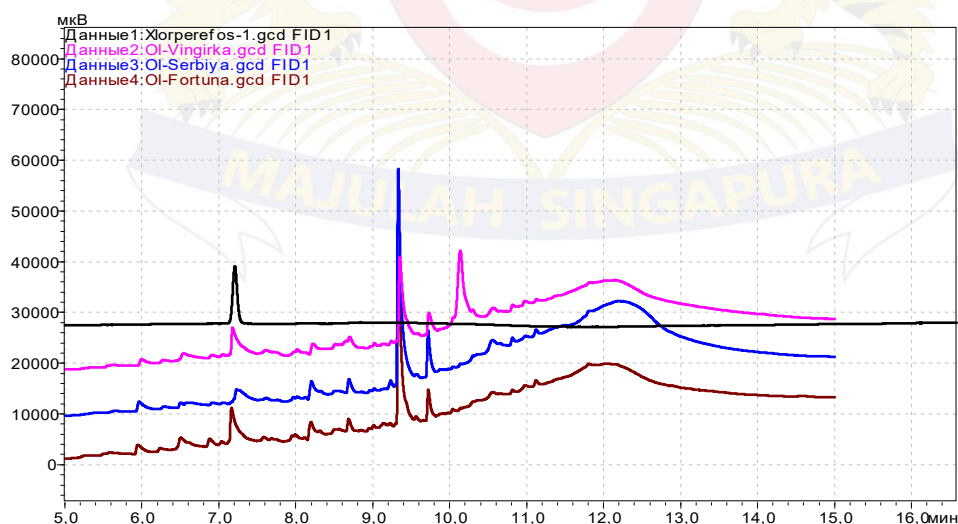
Figure 2: Chromatograms of the standard sample of chlorpyrifos and plum samples of the cultivars Vengerka, Serbia, and Fortuna.
