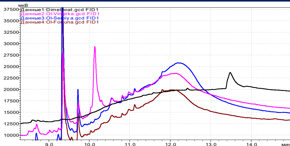
Figure 3: Chromatograms of Dimethoate Pesticide and Samples Belonging to the Hungarian, Serbian, and Fortuna Plum Cultivars
